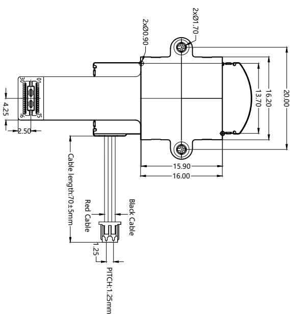
BOTTOM VIEW
